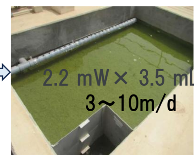
Slow Sand Filter
